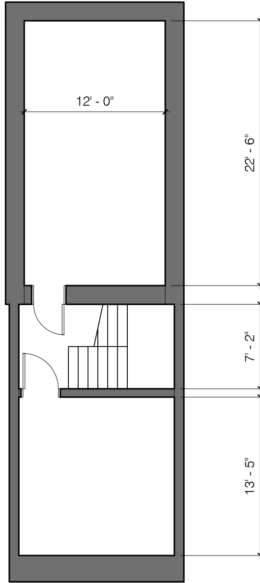
1 BASEMENT 003 1/8" = 1'-0"
